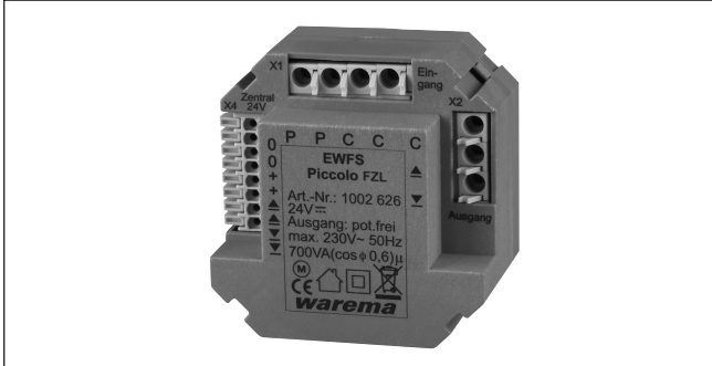
Abb. 1 EWFS Piccolo FZL
